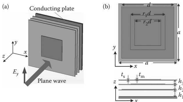
Figure 5.4 Reflecting element characterizing three-layer stacked square patches of variable size. (a) Oblique view. (b) Elevation view and side view. In the elevation view, the second and third substrate layers are omitted to show all the three patch layers clearly.
