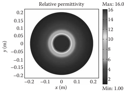
Figure 7.37 Dielectric permittivity distribution for the black hole.
