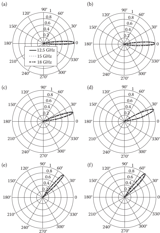
Figure 8.25 Measured far-field results of the 3D lens. (a, c, e) Horizontal polarizations and (b, d, f) vertical polarizations at 12.5, 15, and 18 GHz. (a, b) The feeding source is located at the center of the focal plane ( x = 0 and y = 0 ). (c, d) The feeding source is 10 mm off the center of the focal plane ( x = -10 mm and y = 0 ). (e, f) The feeding source is 30 mm off the center of the focal plane. (Reprinted by permission from Macmillan Publishers Ltd. Nat. Commun. H. F. Ma and T. J. Cui. Three-dimensional broadband and broad-angle transformation-optics lens. 1: 124. Copyright 2010.)
