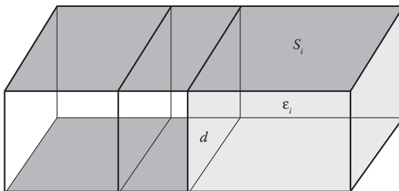
Figure 7.3 Parallel capacitor model.
