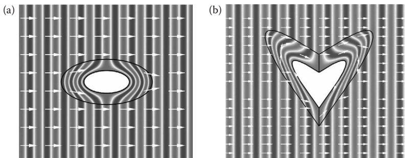
Figure 6.6 Near-field distributions of (a) elliptical-cylindrical cloak and (b) heart-shaped invisibility cloak.
