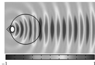
Figure 7.14 Simulated electric field distribution of the 2D Luneburg lens.
