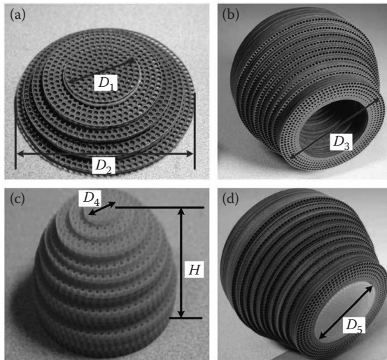
Figure 3.14 Construction of a 3D flatten Luneburg lens fabricated with multilayered dielectric plates by drilling inhomogeneous holes. (a) The first region (the top part) was fabricated using 2 \times 2 \times 1 \text{ mm}^3 F4B unit cells. (b) The second region (the bottom shell) was fabricated using 2 \times 2 \times 2 \text{ mm}^3 F4B unit cells. (c) The third region (the bottom core) was fabricated using 2 \times 2 \times 2 \text{ mm}^3 FR4 unit cells. (d) Construction of the whole lens. (Reprinted by permission from Macmillan Publishers Ltd. Nat. Commun. H. F. Ma and T. J. Cui. Three-dimensional broadband and broad-angle transformation-optics lens. 1: 124. Copyright 2010.)
