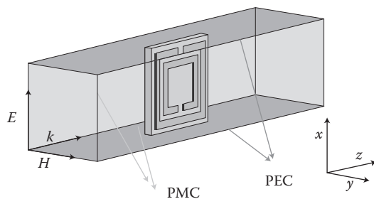
Figure 2.6 Waveguide method used for the simulation of the metamaterial unit cell.
