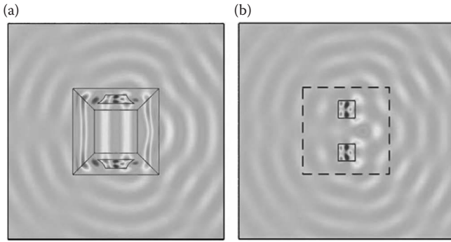
Figure 6.12 The scattering field of (a) a metallic square object with an illusion device in real space and (b) two dielectric square objects in virtual space. (Reprinted with permission from W. X. Jiang, H. F. Ma, Q. Cheng, and T. J. Cui. Illusion media: Generating virtual objects using realizable metamaterials. Appl. Phys. Lett. , 96: 121910. Copyright 2010, American Institute of Physics.)
