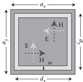
Figure 7.28 Structure of the closed square ring.
