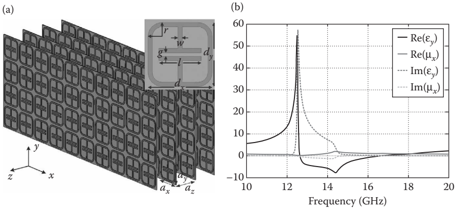
Figure 4.5 (a) Visualization of metamaterial formed by periodic arrangement of ELC resonators (ELCRs), where a_x , a_y , and a_z are the lattice constants. The geometric parameters of ELCR: d_x , d_y , r , l , w , and g are defined in the inset. (b) Frequency response of effective relative permittivity \epsilon_y and permeability \mu_x for ELCR-based metamaterial with the following specifications: a_x = a_y = a_z = 3.333 mm, d_x = d_y = 3 mm, r = 0 mm, l = 1 mm, w = 0.25 mm, g = 0.25 mm, t_m = 0.017 mm, \sigma_m = 5.8 \times 10^7 S/m, t_s = 0.203 mm, Dk = 3.75 , and Df = 0.02 .
