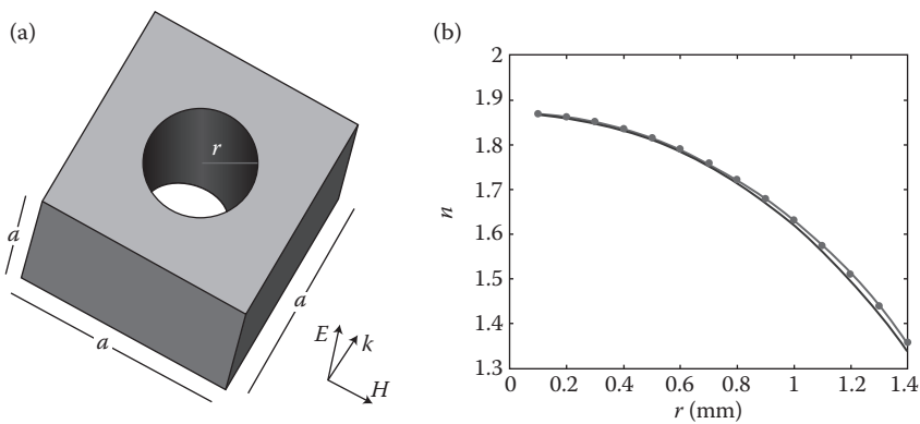
Figure 7.8 Geometry of the unit cell (a) and the effective refractive index variation along with the radius of the hole (b).
