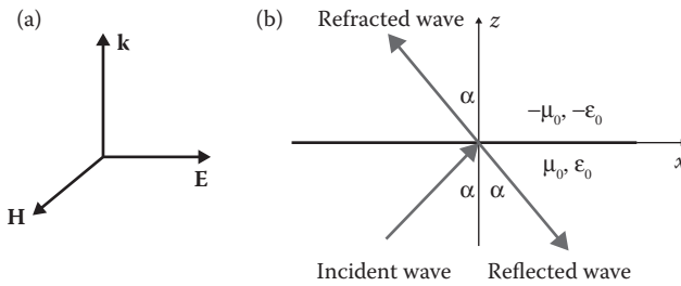
Figure 1.1 (a) The electric field, magnetic field, and propagation vector form a left-handed system. (b) The reflection and refraction features of electromagnetic wave on the interface of right-handed and left-handed materials, in which negative refraction is observed.
