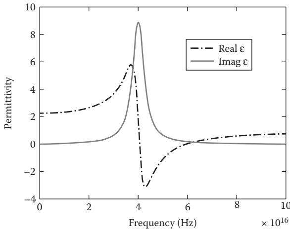
Figure 2.2 A typical Lorentz–Drude dispersion curve for natural materials.
