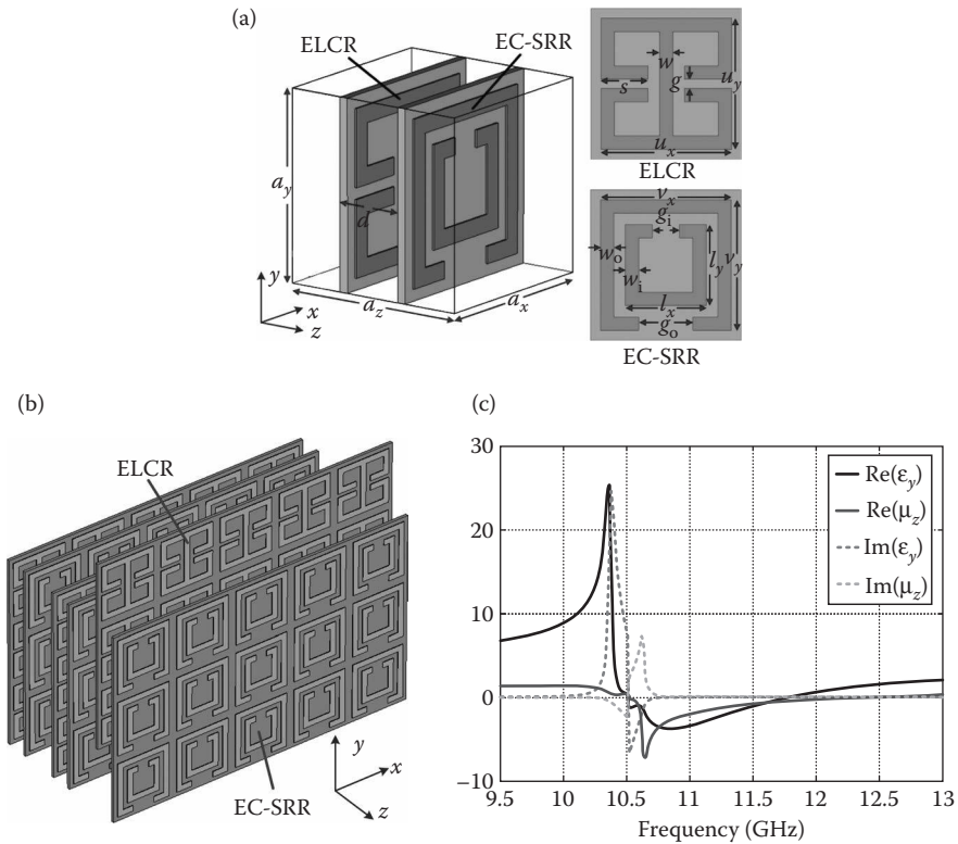
Figure 4.11 (a) Cubic lattice of DNG metamaterial formed by periodic arrangement of pairs of ELCR and EC-SRR, where a_x , a_y , and a_z are the lattice constants, d is the spacing between the ELCR and EC-SRR planes within a cell, u_x , u_y , s , w , and g are the geometric parameters of ELCR, and v_x , v_y , l_x , l_y , w_o , w_i , g_o , and g_i are the geometric parameters of EC-SRR. (b) Visualization of DNG metamaterial combining ELCRs and EC-SRRs. (c) Frequency response of effective relative permittivity \epsilon_y and permeability \mu_z for DNG metamaterial combining ELCRs and EC-SRRs with the following specifications: a_x = a_y = a_z = 3.333 mm, d = 1.67 mm, u_x = u_z = 2.9 mm, g = 0.2 mm, s = 1.05 mm, w = 0.3 mm, v_x = v_z = 2.9 mm, l_x = l_z = 1.8 mm, g_i = 0.6 mm, g_o = 1.2 mm, w_o = w_i = 0.3 mm, t_m = 0.035 mm, \sigma_m = 5.8 \times 10^7 S/m, t_s = 0.35 mm, Dk = 2.33 , and Df = 0.003 .
