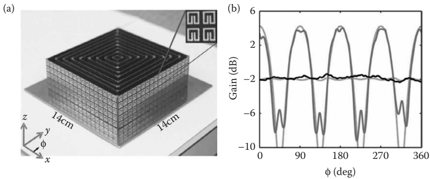
Figure 6.10 (a) Photograph of the fabricated broadband transformation optics lens. (b) Simulated and measured gain patterns of the monopole with and without the transformation optics lens. (Reprinted with permission from Z. H. Jiang, M. D. Gregory, and D. H. Werner, Phys. Rev. B , 84: 165111. Copyright 2009 by the American Physical Society.)
