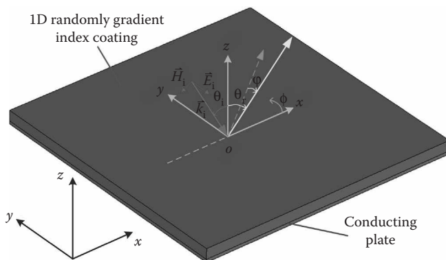
Figure 5.6 An infinite s-polarized plane wave incident on a 1D randomly gradient index coating backed with a PEC plate. The solid dark arrow represents the incident direction and the dashed dark arrow represents the specular direction.
