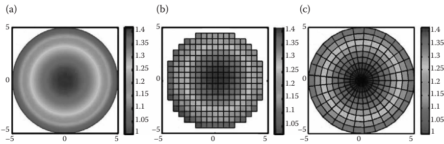
Figure 7.12 Refractive index profile for 2D Luneburg lens. (a) Continuous distribution, (b) discrete distribution in the rectangular grid, (c) discrete distribution in the polar grid.
