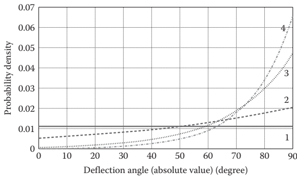
Figure 5.8 Probability density functions of local-beam deflection angles for different random distribution modes. The solid curve marked 1 represents the uniform distribution and the rest three curves correspond to three nonuniform distributions, respectively. (X. M. Yang, Q. Cheng, and T. J. Cui, Research on the one-dimensional randomly gradient index coating. In Proceedings of the 2010 International Conference on Microwave and Millimeter Wave Technology , Chengdu, China, 1208–1211 © 2010 IEEE.)
