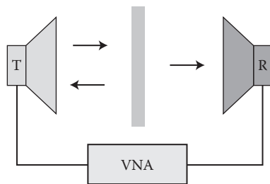
Figure 2.5 Schematic demonstration of the measurement system.
