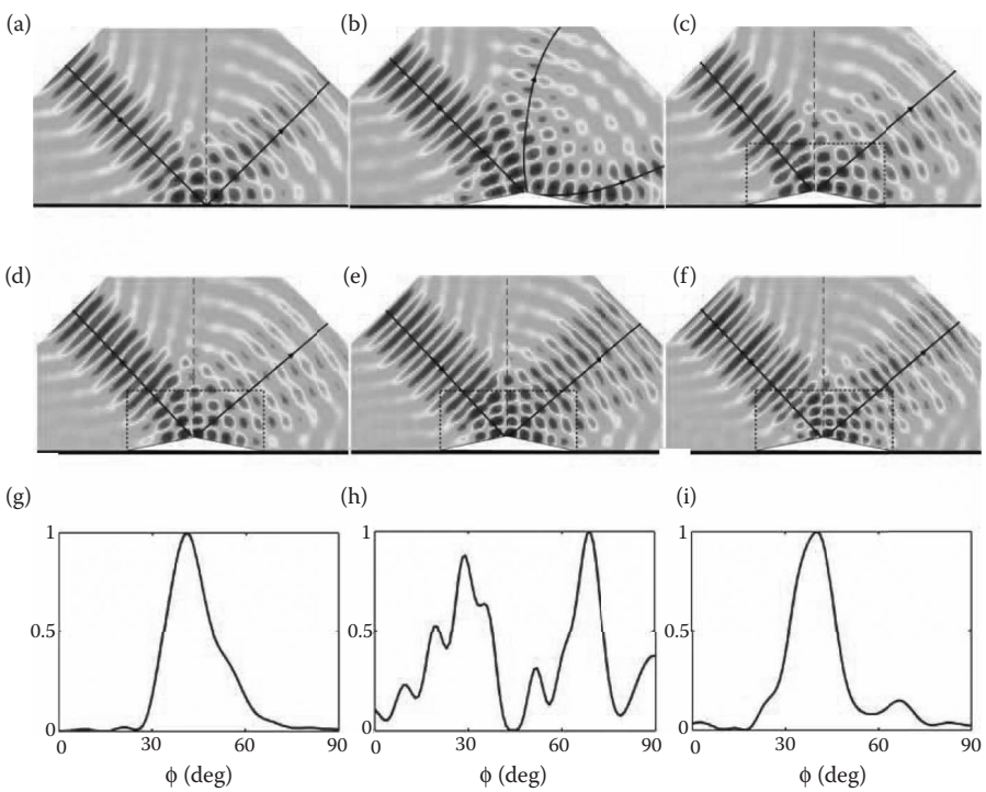
Figure 8.10 Measured electric field mapping of (a) the ground plane, (b) triangular metallic bump, and (c) ground-plane cloaked bump when collimated beam is incident at 10 GHz. The rays display the wave propagation direction, and the dashed line indicates the normal of the ground in free space and that of the ground-plane cloak in the transformed space. (d–f) Collimated beam incident on the ground-plane cloaked bump at 11, 12, and 13 GHz, respectively. Far-field patterns when collimated beam is incident at 10 GHz on (g) the ground plane, (h) the triangular metallic bump, (i) the ground-plane cloaked bump. (From H. F. Ma et al. Compact-sized and broadband carpet cloak and free-space cloak. Opt. Express , 17: 19947, 2009. With permission of Optical Society of America.)
