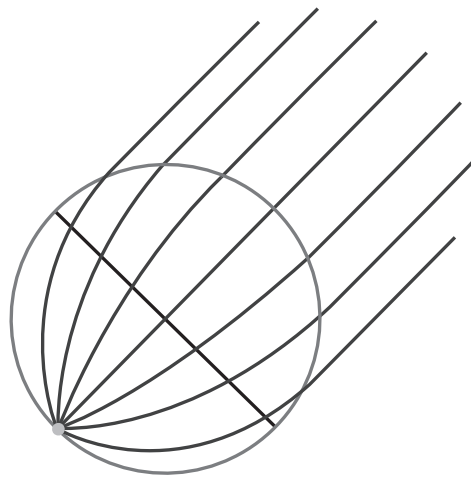
Figure 7.13 Ray trajectories of the 2D Luneburg lens.
