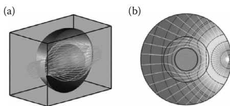
Figure 3.20 The principle of D.C. invisibility cloak. (a) The currents distribution when the object is covered by the cloak. The cloak smoothly guides the electric currents around the inner object and turns them back to the original direction. (b) The equipotential lines and current density vectors on a cross section when the cloaked object is illuminated by a point source, in which the white curves denote the current density vectors and the black curves represent the equipotential lines. (Reprinted with permission from F. Yang et al., Phys. Rev. Lett. , 109: 053902. Copyright 2012 by the American Physical Society.)
