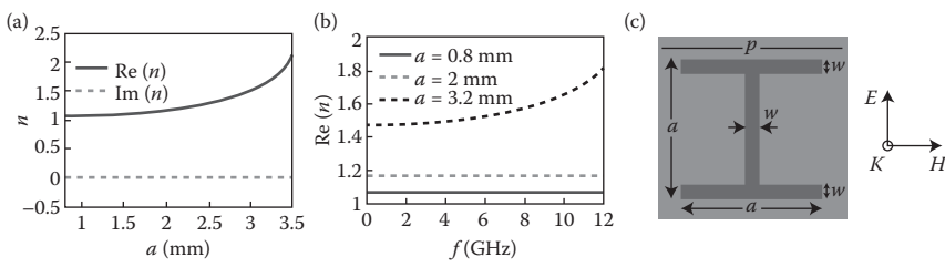
Figure 7.20 Variation of retrieved EM parameters with the geometrical size (a), dispersion of the I-shaped unit cell (b), and the cell structure (c).
